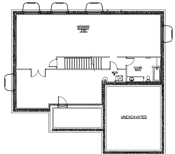
Unfinished Basement 1,882 sq ft
