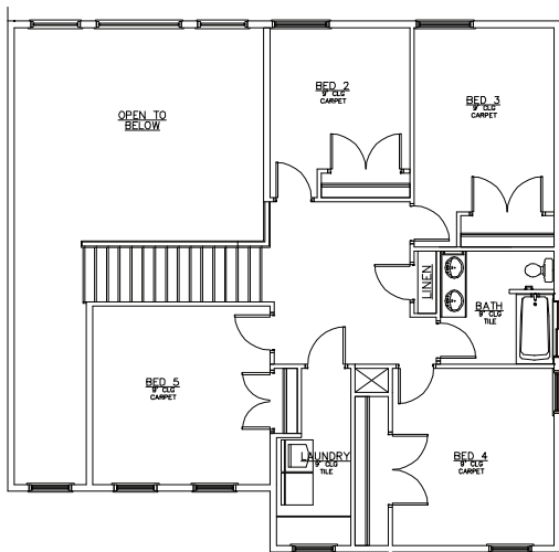
Second Floor 995 sq ft
