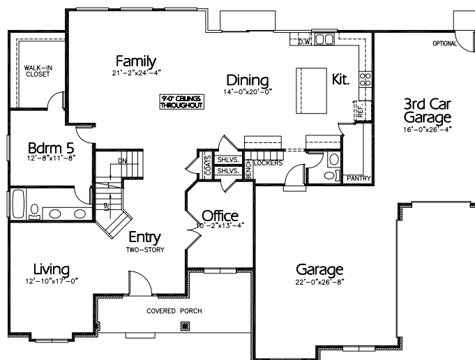
Main Floor 2,149 sq ft
