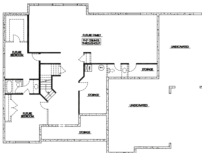
Unfinished Basement 2,303 sq ft
