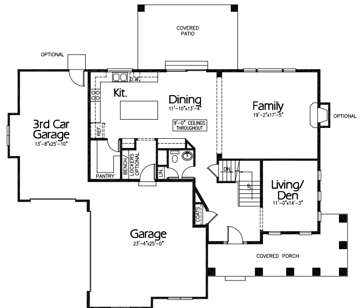
Main Floor 1,333 sq ft
